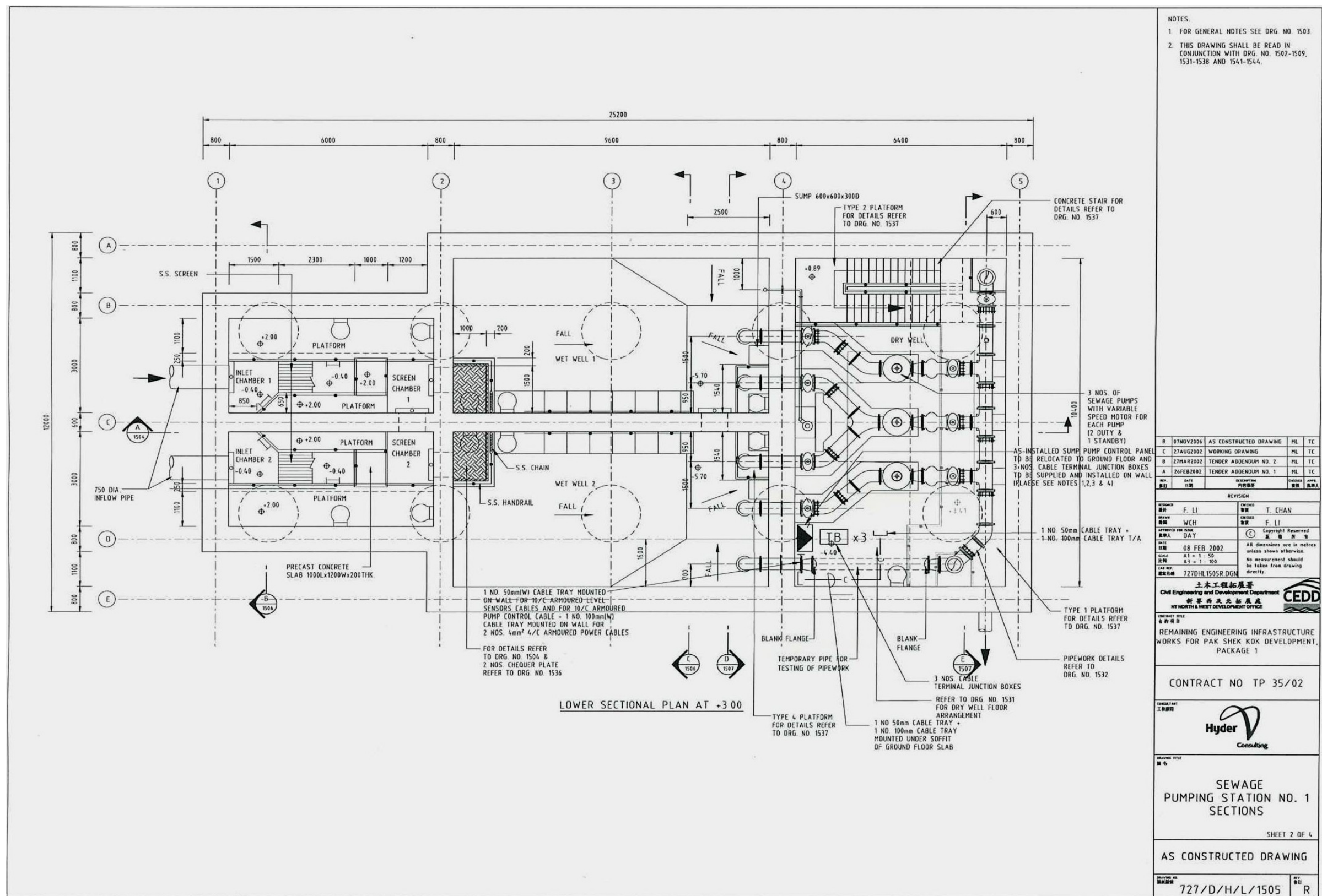
Figure 5: Sewage Pumping Station No. 1 Sections
